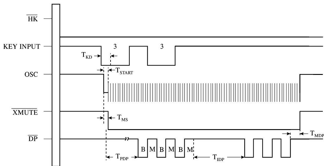
Figure 2. Pulse Mode
