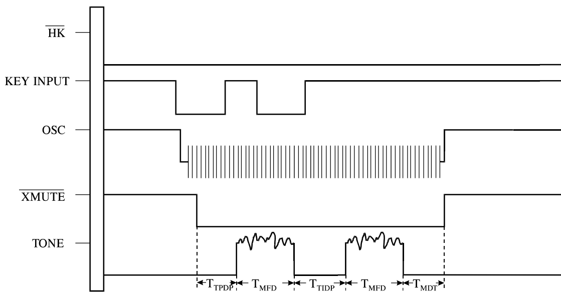
Figure 3. Tone Mode
